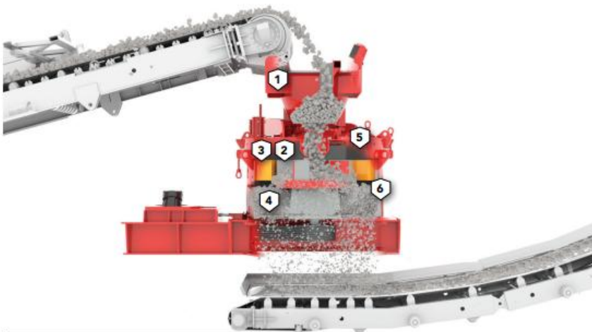
VERTICAL IMPACT CRUSHER IN USE
